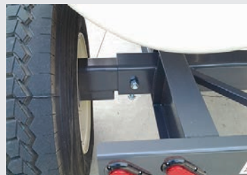
Standard adjustable rear axle from 102" to 120" includes tension bolts on bottom of tube for extra reinforcement.
